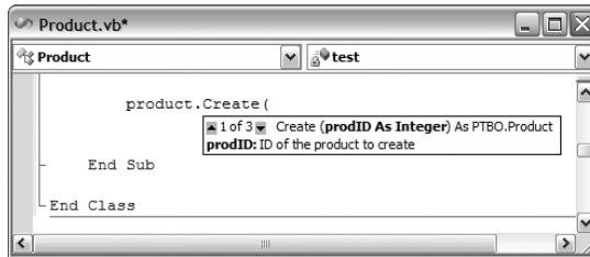
Figure 5.2 The 1 of 3 advises you that this method has three overloads. Use the up and down arrows to show the Parameter Info for each overloaded method.
