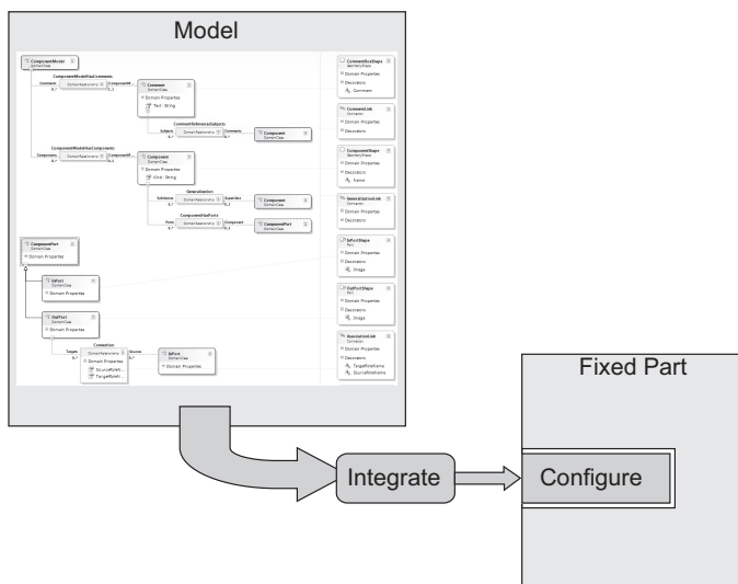
FIGURE 1-1: Domain-Specific Development
