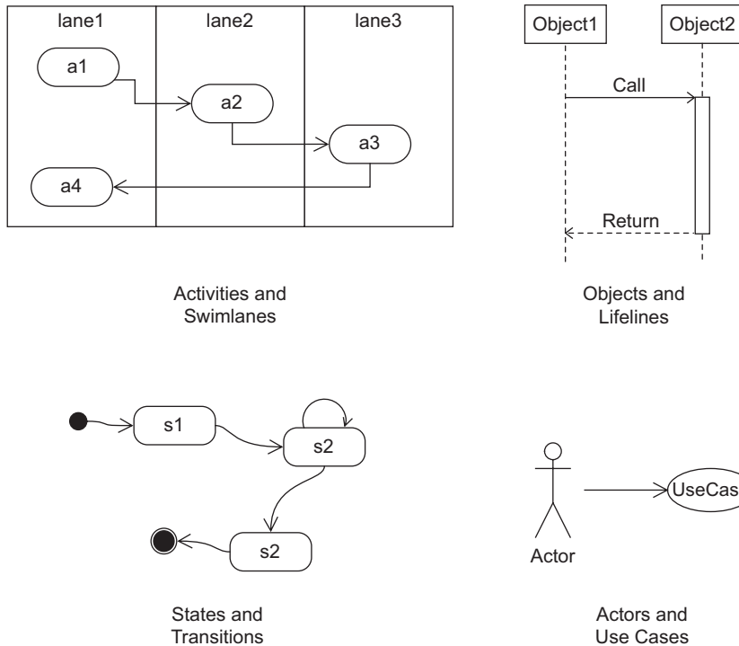
FIGURE 1-12: Behavioral conventions
