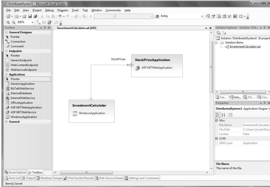
FIGURE 1-14: An application diagram
