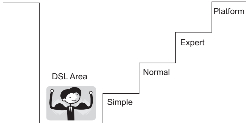
FIGURE 1-17: Customization staircase
