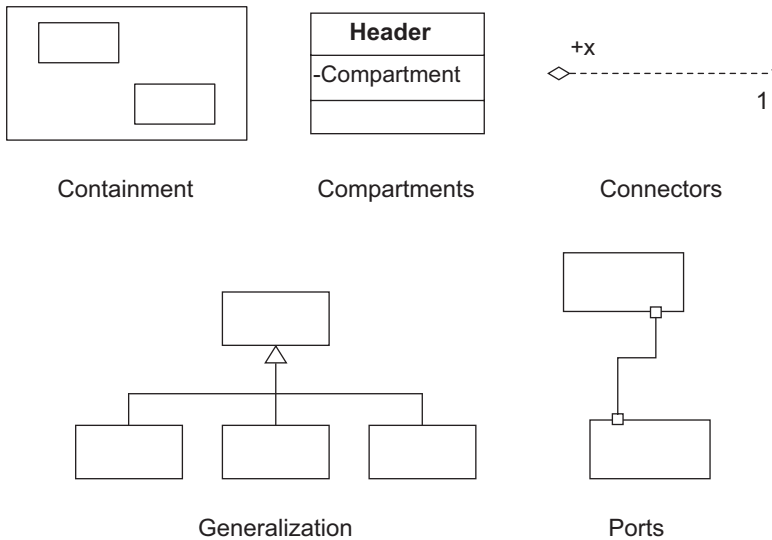
FIGURE 1-11: Structural conventions
