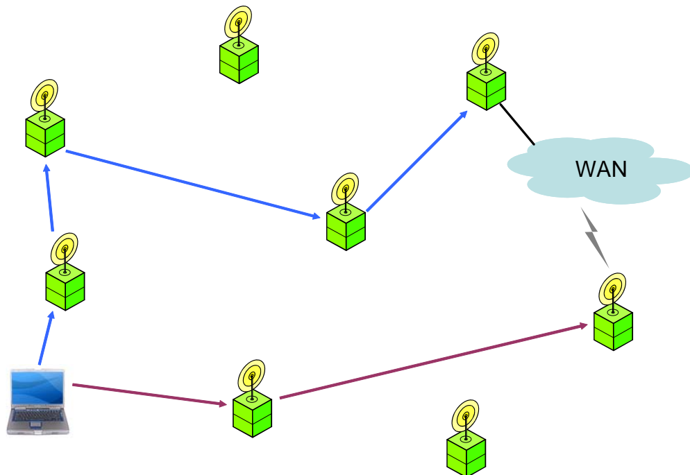
Figure 1 - A key characteristic and advantage to the mesh approach is dynamic routing, improving capacity, resilience, and time-bounded performance. Note multiple paths through the mesh. But adding capacity can involve more nodes and more radios per node, increasing the potential for interference to unrelated nearby Wi-Fi networks. Source: Farpoint Group.
